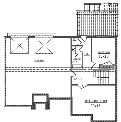
BASEMENT PLAN
